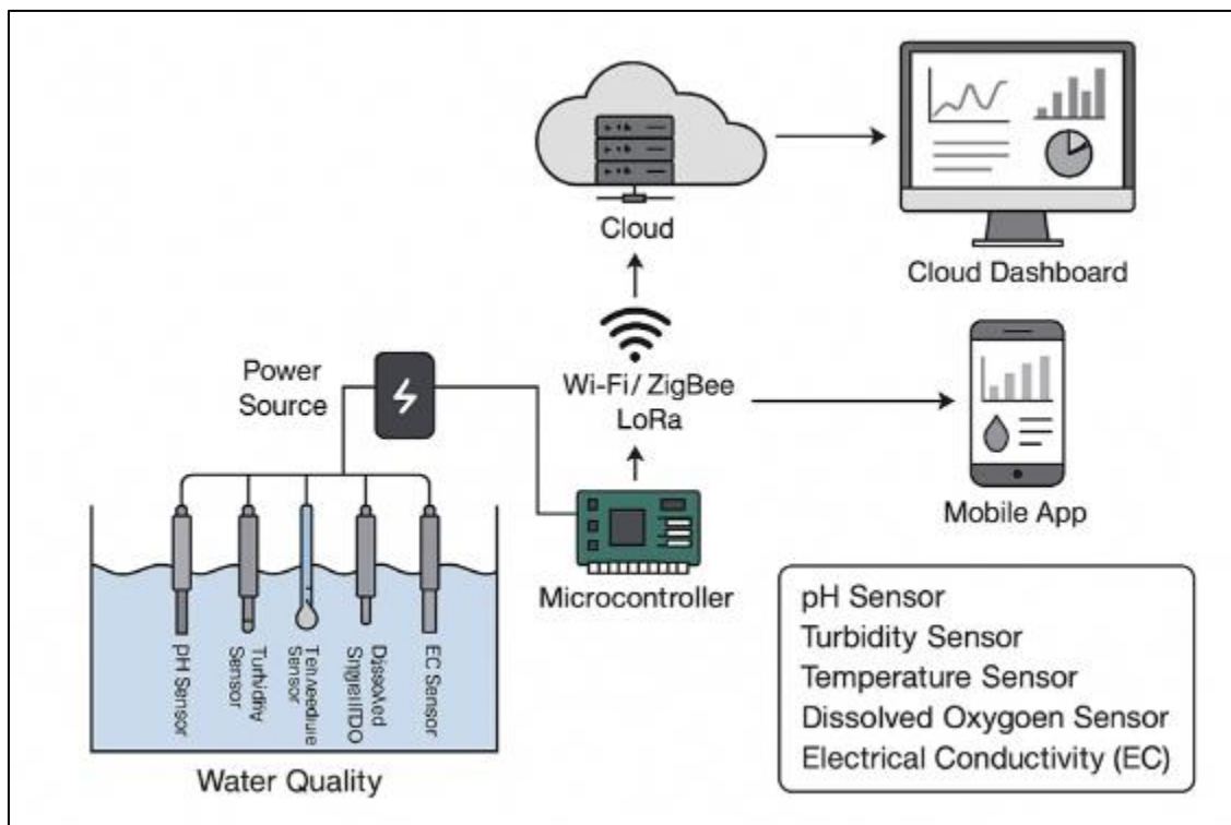
Figure 2: IoT-based water quality monitoring system
